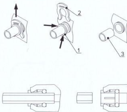
Figure 7. Disconnection of tubes
