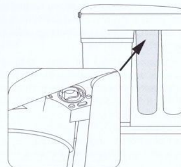
Figure 12. Installation of the membrane cartridge service plug
